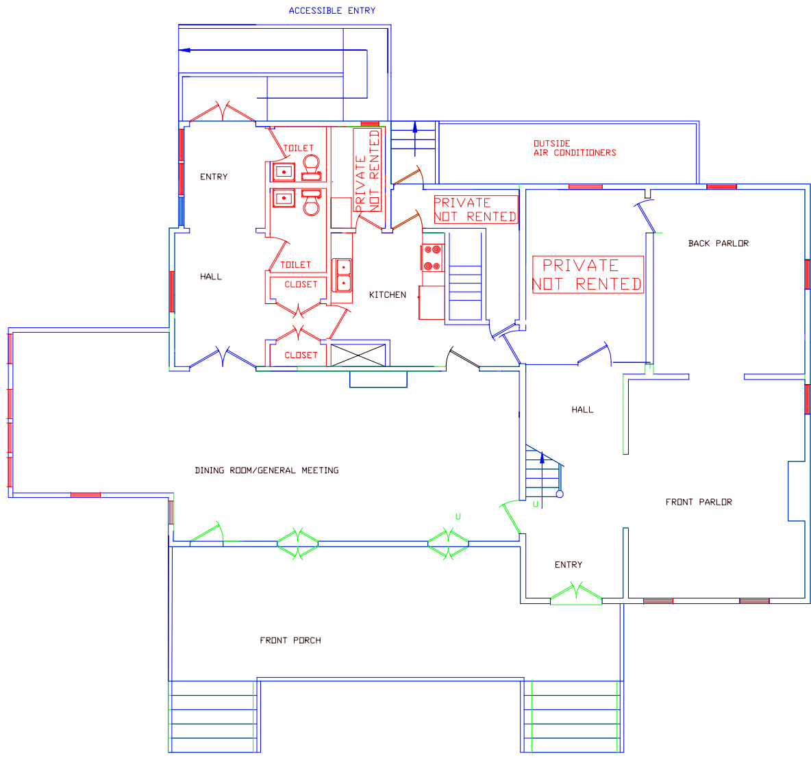
FIRST FLOOR PLAN AFTER 2000 RENOVATION
